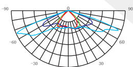
Type 2 FWHM 140° x 70°
