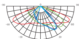
Type 3 FWHM 140° x 70°
